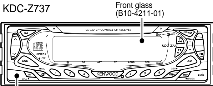
Panel assy (A64-2648-11)
