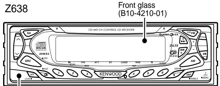
Panel assy (A64-2647-11)
